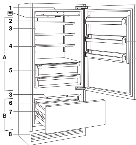
CombiCooler V6000 Supreme
